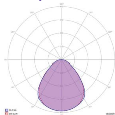
light distribution
